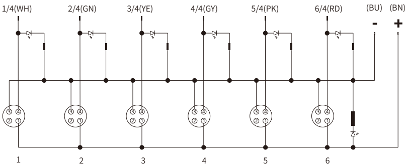
LED indicating: PNP other circuit diagram (NPN) can be customized
